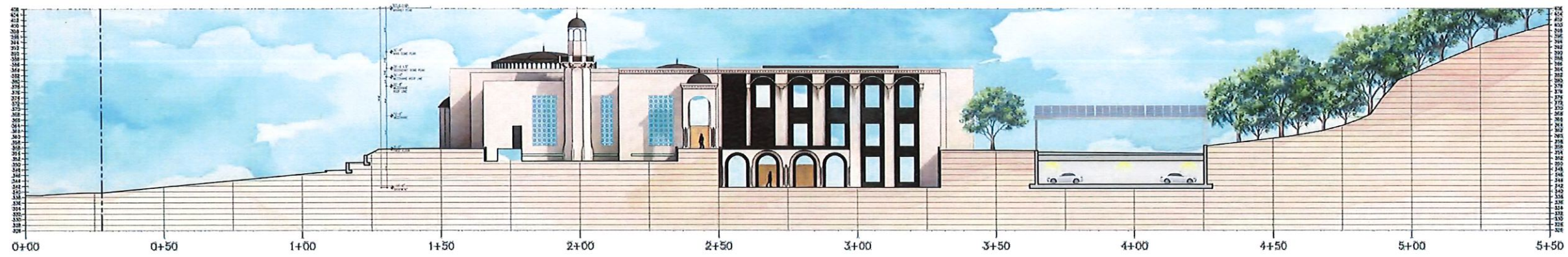
PROPOSED RENDERED SITE SECTION SCALE: 1"=20'-0"
