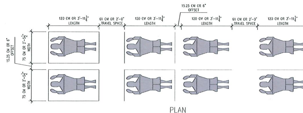
3 PRAYER SEAT DIAGRAM A-102 SCALE: 1/2" = 1'-0"
