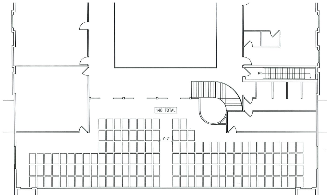
2 ENLARGED MEZZANINE SEATING PLAN A-102 SCALE: 1/8" = 1'-0"
