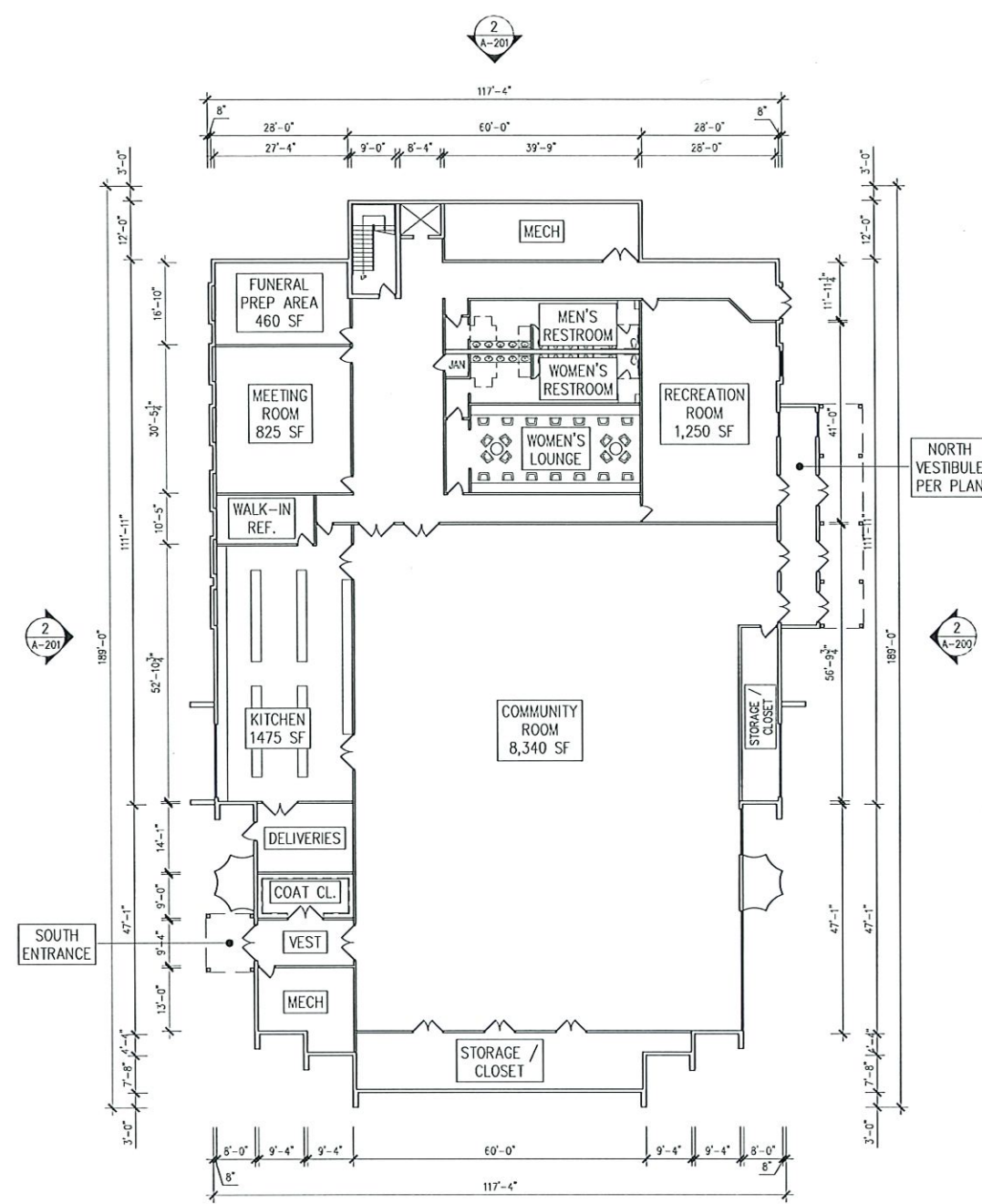
1 BASEMENT FLOOR SCALE: 1/16" = 1'-0"
