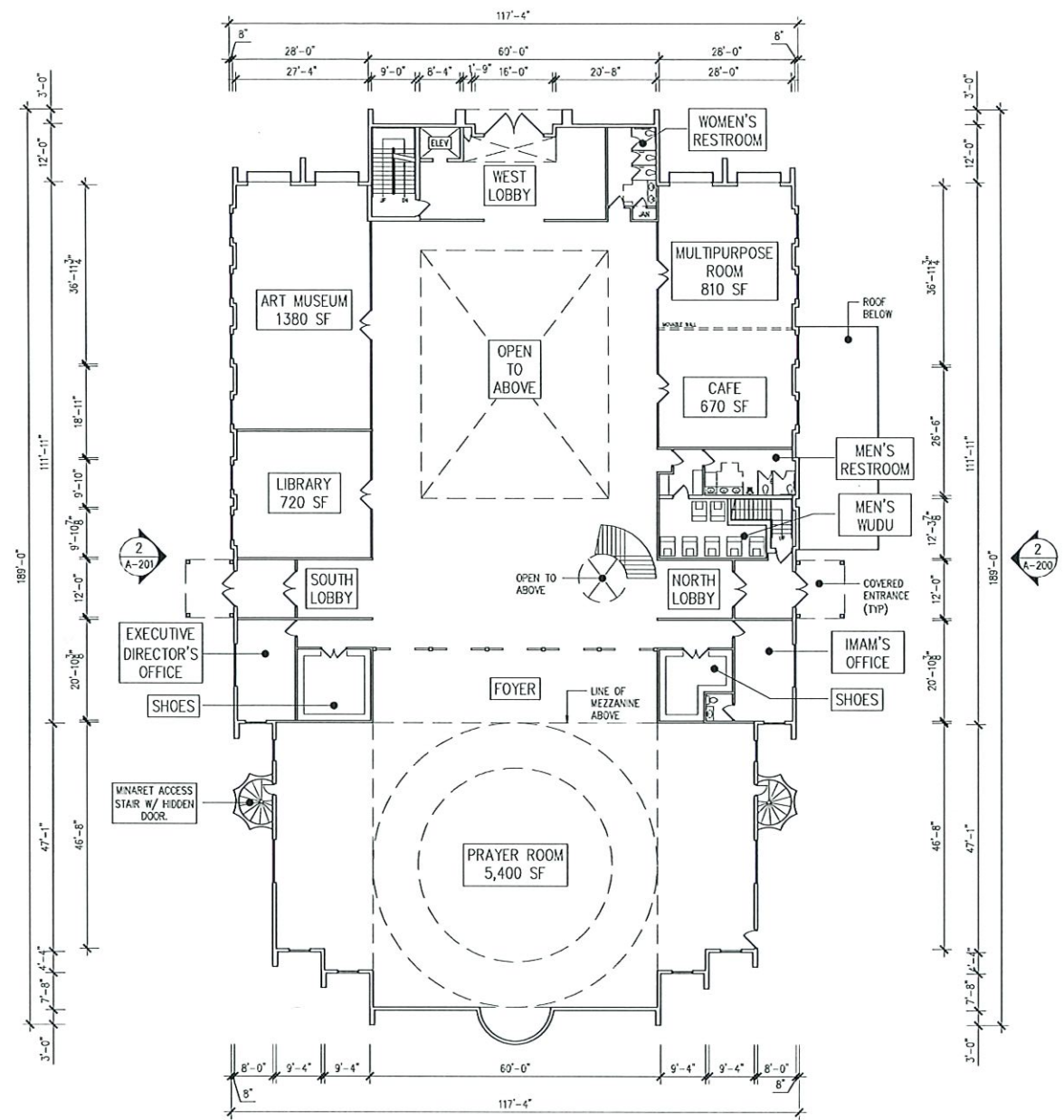
2 FIRST FLOOR SCALE: 1/16" = 1'-0"
